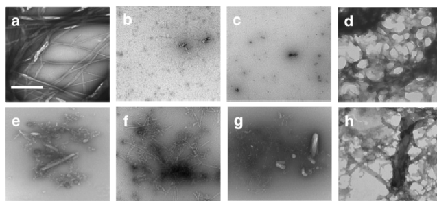
Figure 3. Inhibition experiments. TEM images of samples of Cu ^{\text{II}} -treated A \beta (a) incubated with the chelator [(b) 1 , (c) 2 , (d) CQ, (e) EDTA, or (f) phen] or with the control molecule [(g) MPY or (h) stilbene] ([A \beta ] = 25 \mu\text{M} , [Cu ^{\text{II}} ] = 25 \mu\text{M} , [chelator] = 50 \mu\text{M} , 24 h, 37 ^\circ\text{C} , constant agitation). The scale bar indicates 500 nm.
