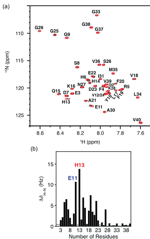
Figure 2. NMR studies of A \beta with 2 . (a) Overlay of 2D TROSY ^1\text{H} – ^{15}\text{N} HSQC spectra of A \beta upon addition of 2 (900 MHz, 200 mM SDS, 20 mM sodium phosphate, pH 7.3, 25 ^\circ\text{C} ). Black and red chemical shifts were obtained from the A \beta sample ( ^{15}\text{N} -labeled A \beta_{1-40} was used, ca. 192 \mu\text{M} ) containing ca. 2 \mu\text{L} of DMSO- d_6 or ca. 1.2 equiv of 2 (ca. 1.4 \mu\text{L} DMSO- d_6 ), respectively. (b) Change in the combined ^1\text{H} and ^{15}\text{N} chemical shifts as a function of the amino acid sequence to identify the major interaction sites of A \beta with 2 . * Denotes absent or overlapped signals.
