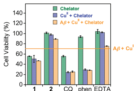
Figure 4. Cytotoxicity of Cu-associated \text{A}\beta with the chelators in SK-N-BE(2)-M17 cells using a MTT assay. Cell viability (%) with [chelator] (green), [the chelator and \text{Cu}^{\text{II}} ] (blue), or [ \text{Cu}^{\text{II}} , \text{A}\beta , and chelator] (orange) after 24 h incubation ( [\text{A}\beta] = 20 \mu\text{M} , [\text{Cu}^{\text{II}}] = 20 \mu\text{M} , [chelator] = 40 \mu\text{M} ). Treatment of \text{A}\beta in the absence and presence of \text{Cu}^{\text{II}} for 24 h results in \sim 90 and \sim 70\% survival of cells, respectively.
