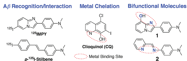
Figure 1. Strategy of designing bifunctional small molecules. Chemical structures of 125 IMPY, p - 125 I-stilbene, CQ, 1 , and 2 are depicted.
