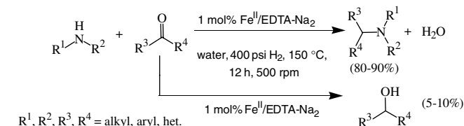
Scheme 1. DRA of carbonyl compounds with amines catalyzed by Fe II /EDTA.
