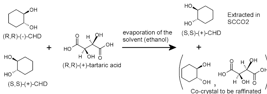
Fig. 1. Scheme of the resolution of (±)-CHD by co-crystal formation followed by an extraction in CO 2 [12].
