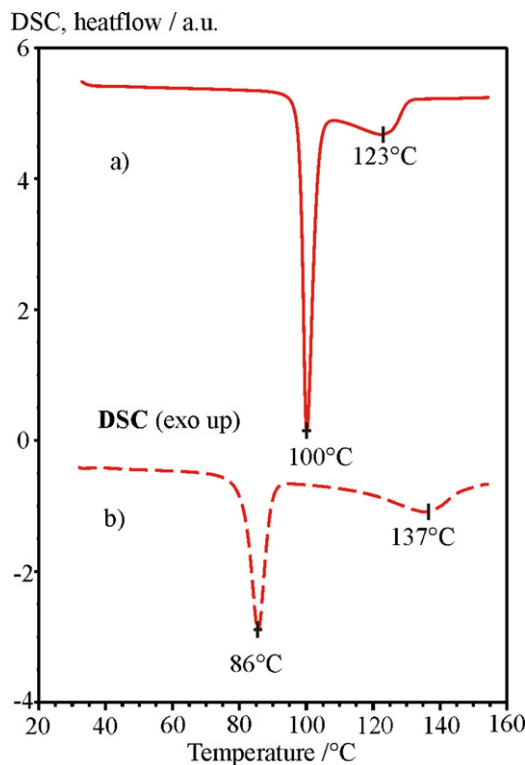
Fig. 8. DSC curve of binary mixtures corresponding to 1:1 molar ratio of –a) ( R,R )-CHD and co-crystal ( 1 ) and b) ( S,S )-CHD and ( R,R )-TA, both exhibiting eutectic melting behavior.
