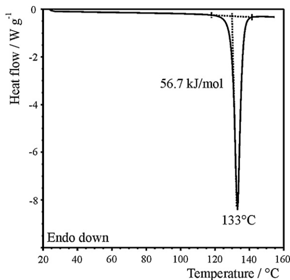
Fig. 6. DSC melting peak of the pure CHD-TA co-crystal ( 1 ) in sealed Al-pan at 10 °C/min (mass 2.59 mg).
