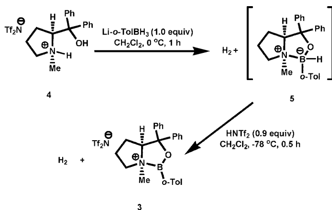
Scheme 1. Preparation of Catalyst 3
