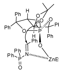
Fig. 2 Model for the hydrophosphonylation of N -diphenylphosphinoyl imines with ( R,R )-TADDOL phosphite 3 .
