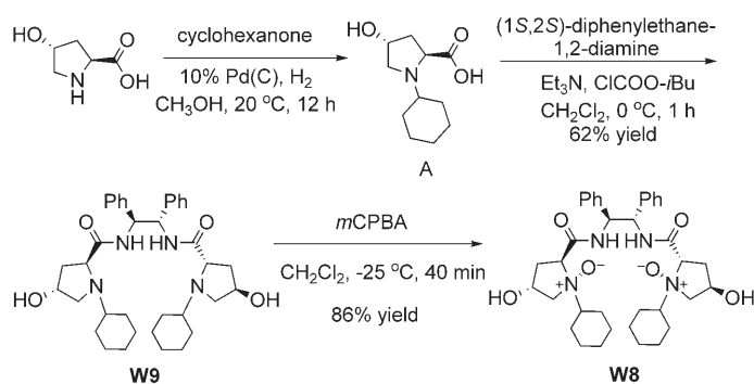
Scheme 2. Synthesis of the chiral catalyst W8 from trans -4-hydroxy-L-proline.
