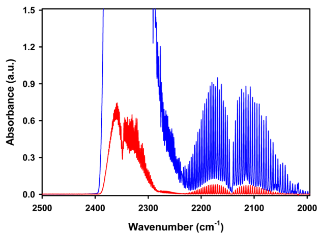
Figure 5. (Blue) Infrared spectrum of gas-phase products after photolysis ( \lambda > 305 \text{ nm} ) of glyoxylic acid for 8 h. All other experimental conditions are indicated in Figure 1. The red trace shows a 1:18 dilution of the spectrum.
