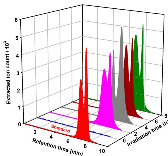
Figure 4. UHPLC-MS for the extracted ion at m/z 417.05 for (E) and (Z) DNPH-glyoxal hydrazones in the experiment of Figure 1. The red trace corresponds to a standard.
