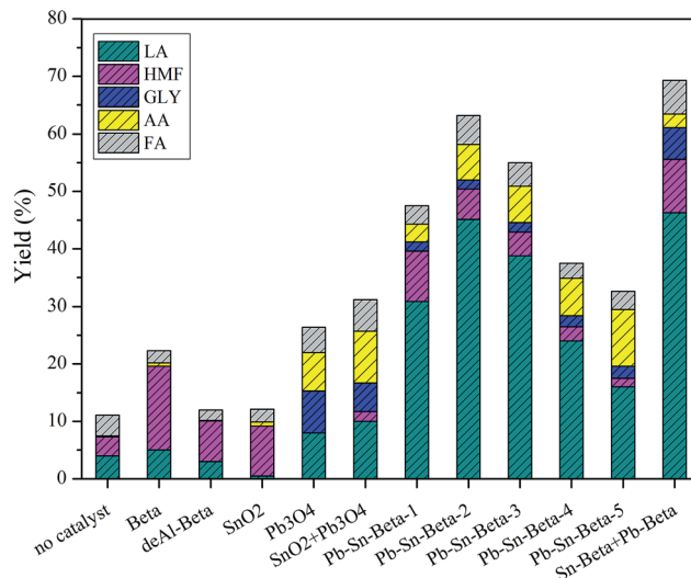
Fig. 1 Comparison of different catalysts for the conversion of glucose. Reaction conditions: 190 °C, 2 h, air, 225 mg glucose and 200 mg catalyst. LA: lactic acid, AA: acetic acid, FA: formic acid, and GLY: glycolic acid. Metal content of Sn-beta + Pb-beta: Sn = 0.2 mmol g -1 , Pb = 0.2 mmol g -1 .
