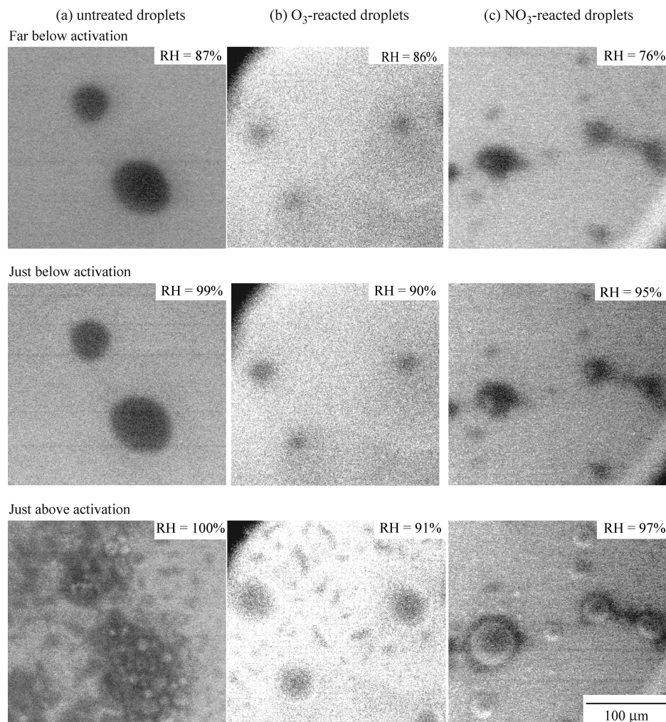
Figure 3. Micrographs obtained by environmental scanning electron microscopy (ESEM). Columns show images collected of (a) untreated oleic acid droplets, (b) \text{O}_3 -treated droplets (method 1; see section 2.4), and (c) \text{NO}_3 -treated droplets (method 2). Rows, shown for increasing relative humidity, reveal that hygroscopic droplet growth occurs at an activation relative humidity. The precise humidity depends on droplet treatment (i.e., \text{O}_3 or \text{NO}_3 exposure). Conditions: (b) exposure to 90 min of 300 ppm \text{O}_3 followed by 3 days storage and (c) exposure to \text{NO}_3 as “low \text{NO}_3 ” (224 min) \rightarrow “high \text{NO}_3 ” (55 min) \rightarrow “low \text{NO}_3 ” (52 min) \rightarrow 0 ppm (70 min) followed by two months storage. The images are adjusted in Adobe Photoshop to improve contrast and brightness.
