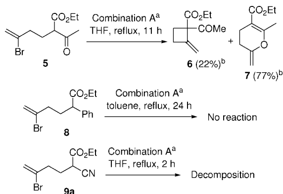
Scheme 1. Reactions of Esters 5 , 8 , and 9a a,b
