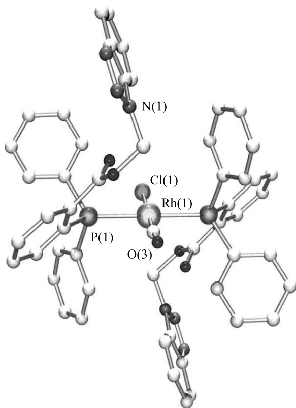
Fig. 4. Molecular structure of \text{Rh}(\text{CO})\text{Cl}[\text{C}_6\text{H}_4\text{N}_3\text{CH}_2\text{CO}_2\text{C}_6\text{H}_4\text{P}(\text{C}_6\text{H}_5)_2]_2 ( 8 ).
