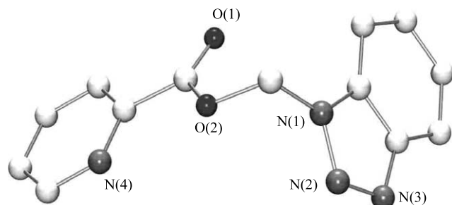
Fig. 1. Molecular structure of ( \text{C}_6\text{H}_4\text{N}_3\text{CH}_2\text{CO}_2\text{C}_5\text{H}_4\text{N} ) ( 1 ).
