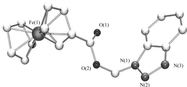
Fig. 2. Molecular structure of (C 6 H 4 N 3 CH 2 CO 2 C 5 H 4 FeC 5 H 5 ) ( 2 ).
