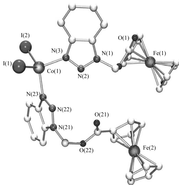
Fig. 3. Molecular structure of \text{CoI}_2(\text{C}_6\text{H}_4\text{N}_3\text{CH}_2\text{CO}_2\text{C}_5\text{H}_4\text{FeC}_5\text{H}_5) ( 6 ).
