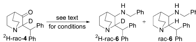
Scheme 3. Use of 2 H- rac - 4 as a probe for assessing the propensity of (2 S )- 4 to epimerize during reductive amination
