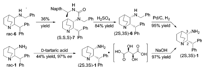
Scheme 2. Literature methods for the isolation of primary amine (2 S ,3 S )- 1
