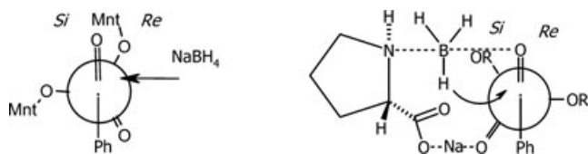
FIGURE 2 Facial attack on the \alpha -phenylketophosphonate carbonyl group by \text{NaBH}_4 (left) and \text{NaBH}_4\text{-Pro} (right).
