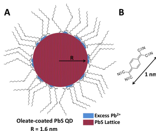
Figure 1. (A) Cartoon of oleate-coated PbS QDs showing submonolayer coverage of the stoichiometric PbS surface with excess Pb 2+ . NMR measurements indicate that there are approximately 150 oleate ligands/PbS QD ( \sim 4.8 oleate ligands/nm 2 ); see Supporting Information. (B) Structure of the electron acceptor tetracyanoquinodimethane (TCNQ).
