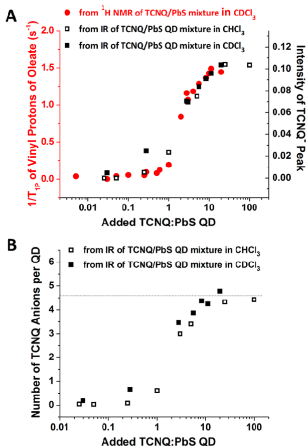
Figure 4. (A) (Left axis, red) Plot of 1/T_{1P} , obtained from eq 1, for vinyl protons (5.3 ppm) of oleate on the surfaces of PbS QDs vs molar ratio TCNQ:QD in mixtures of TCNQ and PbS QDs in \text{CDCl}_3 . (Right axis, black) Plot of intensity of the peak corresponding to the C–N stretching mode of reduced TCNQ vs molar ratio TCNQ:PbS in mixtures of TCNQ and PbS QDs in \text{CDCl}_3 (■) and \text{CHCl}_3 (□). The overlap of NMR and IR data sets indicates that electron transfer to TCNQ is responsible for creation of paramagnetic centers at the surface of the QD. (B) Plot of number of reduced TCNQ molecules per QD vs molar ratio TCNQ:QD in mixtures of TCNQ and PbS QDs in \text{CDCl}_3 (■) and \text{CHCl}_3 (□). The Supporting Information details our procedure for determining the number of reduced TCNQ molecules in a sample.
