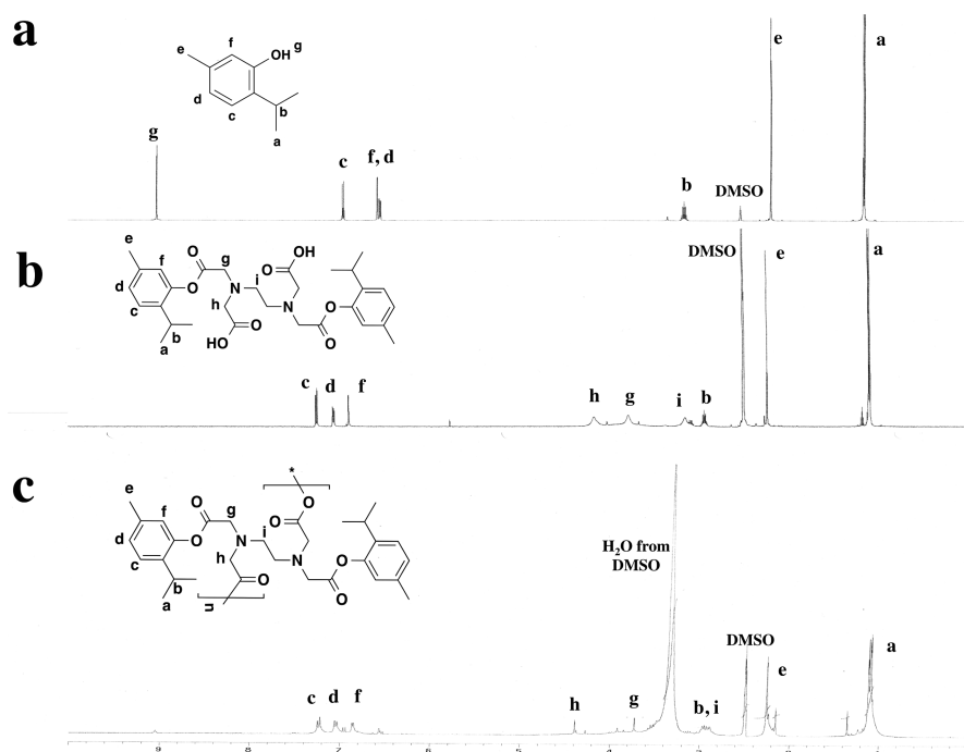
Figure 1. 1 H NMR spectra of thymol (a), corresponding diacid (b), and polymer (c).
