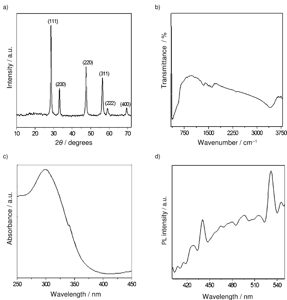
Figure 1. Characterization of CeO 2 nanoparticles prepared via solution combustion method. a) Powder XRD pattern; b) FTIR spectrum; c) UV/Vis spectrum; d) Photoluminescence (PL) spectrum.
