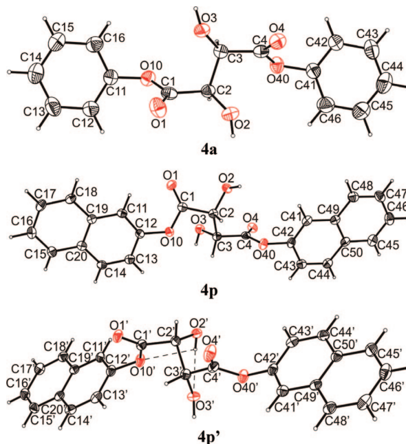
FIGURE 1. Illustration of conformers of the investigated molecules with atom numbering scheme for (4a) T ( sp,sp ), (4p), T ( sp,sp ), and (4p') T ( ap,ap ). Thermal ellipsoids are drawn at 40% probability level. Dashed lines illustrate intramolecular hydrogen bonds; sp and ap refer to relative orientation of the vicinal \text{C}=\text{O} and \text{C}-\text{O}(\text{H}) bonds.
