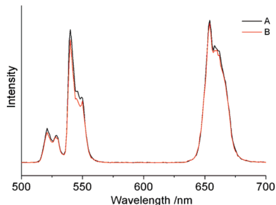
Figure 5. Luminescence spectra of aqueous solutions of NaYF 4 : 20 mol%Yb, 2 mol % Er nanoparticles (0.4 mg/mL) excited with a 980-nm laser: (A) As-prepared sample in cyclohexane; (B) the oxidized sample in water.
