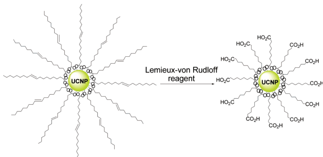
Figure 1. Synthesis mechanism of carboxylic acid-functionalized UCNP from oleic acid-capped precursors.
