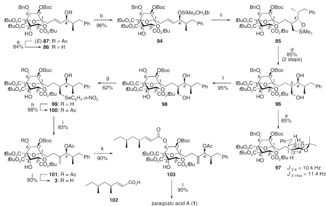
Scheme 8. Conversion of alkene ( E )- 87 to zaragozic acid A (1). a) DIBALH, toluene/CH 2 Cl 2 7:2, -78°C, 1 h; b) ClSiMe 2 CH 2 Br, Et 3 N, DMAP, CH 2 Cl 2 , 0°C, 1 h; c) Bu 3 SnH, AIBN, benzene, reflux, 4 h; d) 35% aq. H 2 O 2 , NaHCO 3 , KF, THF/MeOH 1:1, 24 h; e) TsOH, Me 2 C(OMe) 2 , 1 h; f) H 2 , 20% Pd(OH) 2 /C, AcOEt, 13 h; g) 2-NO 2 C 6 H 4 SeCN, Bu 3 P, THF, 30 min; h) Ac 2 O, DMAP, CH 2 Cl 2 , 0°C, 30 min; i) 35% aq. H 2 O 2 , THF, 4 h; j) 0.2% K 2 CO 3 in MeOH, 1 h; k) carboxylic acid 102 , DCC, DMAP, CH 2 Cl 2 , 5 h; l) TFA, CH 2 Cl 2 , 16 h. DCC = dicyclohexylcarbodiimide.
