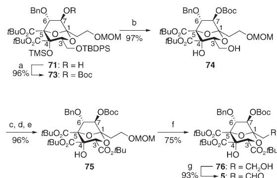
Scheme 6. Synthesis of functionalized core 5 . a) (Boc) 2 O, Et 3 N, DMAP, CH 2 Cl 2 , 2 h; b) Bu 4 NF, THF, 0°C, 30 min; c) Dess–Martin periodinane, CH 2 Cl 2 , 24 h; d) NaClO 2 , NaH 2 PO 4 , 2-methyl-2-butene, t BuOH, H 2 O, 3 h; e) i PrN=C(OrBu)NH i Pr, CH 2 Cl 2 , 48 h; f) TMSCl, Et 4 NBr, CH 2 Cl 2 , 0°C, 1 h, then room temperature, 20 h; g) Dess–Martin periodinane, CH 2 Cl 2 , 30 min.
