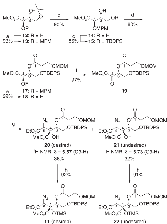
Scheme 2. Synthesis of \alpha -diazo ester 11 . a) MPMOC(NH)CCl 3 , Ph 3 CBF 4 , Et 2 O, 0°C, 30 min; b) 10% aq. HCl, THF, 5 h; c) TBDPSCl, imidazole, CH 2 Cl 2 , 0°C, 1 h; d) EDCI, MOMO(CH 2 ) 2 CO 2 H ( 16 ), DMAP, CH 2 Cl 2 , 12 h; e) DDQ, CH 2 Cl 2 , pH 7 phosphate buffer, 24 h; f) Dess–Martin periodinane, CH 2 Cl 2 , 1 h; g) LiHMDS, N 2 CHCO 2 Et, THF, –78°C, 30 min; h) HMDS, imidazole, THF, 48 h. THF = tetrahydrofuran; EDCI = 1-(3-dimethylaminopropyl)-3-ethylcarbodiimide hydrochloride; DMAP = 4-(dimethylamino)pyridine; HMDS = 1,1,3,3-hexamethyldisilazane.
