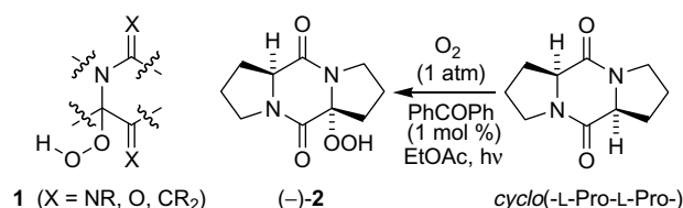
Scheme 1. General formula of organic hydroperoxides 1 and cis -configured L-proline-derived hydroperoxide (–)- 2 . 19
