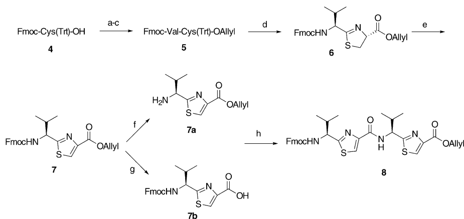
Scheme 2. Synthesis of tetrapeptide 8 . a) HOBt, HBTU, DIEA, allyl alcohol, DMF; b) DEA, \text{CH}_3\text{CN} ; c) HOBt, HBTU, DIEA, N -Fmoc-L-valine, DMF, 84 %; d) \text{Ph}_3\text{PO} , \text{Ti}_2\text{O}_3 , \text{CH}_2\text{Cl}_2 , -20^\circ\text{C} , 89 %; e) activated \text{MnO}_2 , \text{CH}_2\text{Cl}_2 , 94 % (>96 % ee ); f) DEA, \text{CH}_3\text{CN} ; g) \text{Pd}(\text{OAc})_2 , PS-triphenylphosphine, \text{PhSiH}_3 , \text{CH}_2\text{Cl}_2 ; h) HOBt, HBTU, DIEA, DMF, 91 % for f)–h); DEA = N,N -diethylamine, DIEA = N,N -diisopropylethyl-
