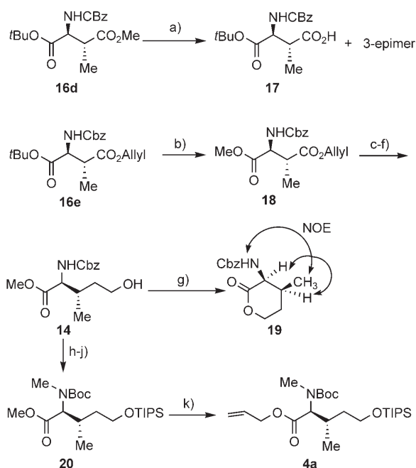
Scheme 5. Second-generation synthesis of the NMeOHlle unit. a) aq. LiOH, MeOH, THF; b) TFA, CH 2 Cl 2 , then CH 2 N 2 , Et 2 O, RT, 95%; c) [Pd(PPh 3 ) 4 ], NMA, CH 2 Cl 2 , RT; d) ClCO 2 iBu, NMM, THF, –20 °C then CH 2 N 2 , Et 2 O, –20 °C → RT; e) AgNO 3 , H 2 O, THF; f) ClCO 2 Et, NMM, THF, 0 °C then NaBH 4 , MeOH, 0 °C → RT 35% yield for 4 steps; g) TsOH·H 2 O, PhH, reflux, 75%; h) TIPSCl, imidazole, DMAP, CH 2 Cl 2 , RT, 89%; i) Pd/C, Boc 2 O, H 2 , MeOH, RT; j) Ag 2 O, MeI, DMF, 50 °C, 94% yield for 2 steps; k) aq. LiOH, THF, MeOH, then allyl bromide, K 2 CO 3 , DMSO, RT, 92%. NMA = N -methylaniline; NMM = N -methylmorpholine; TIPS = triisopropylsilyl.
