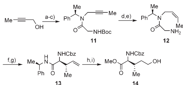
Scheme 3. First-generation synthesis of the NMeOHile unit. a) \text{MsCl} , \text{Et}_3\text{N} , -20^\circ\text{C} \rightarrow \text{RT} ; b) (R) - \alpha -methylbenzylamine, 65% (2 steps); c) N -Boc-Gly, EDCI, HOBT, i\text{Pr}_2\text{NEt} , 0^\circ\text{C} \rightarrow \text{RT} , 96%; d) Lindlar catalyst, \text{H}_2 , ether, RT 91%; e) TFA, \text{CH}_2\text{Cl}_2 , 96%; f) LiHMDS, THF, -78^\circ\text{C} \rightarrow \text{RT} ; g) CbzCl, \text{Et}_3\text{N} , DMAP, \text{CH}_2\text{Cl}_2 , RT, 52% yield for 2 steps; h) HCl (5N), MeOH, reflux, then \text{CH}_2\text{N}_2 , ether, 76%; i) \text{BH}_3 \cdot \text{THF} ; then \text{H}_2\text{O}_2 , pH 7 buffer, 72%; EDCI = 1-(3-dimethylaminopropyl)-3-ethylcarbodiimide hydrochloride; HOBT = 1-hydroxy-1H-benzotriazole; TFA = trifluoroacetic acid; HMDS = hexamethyldisilazide.
