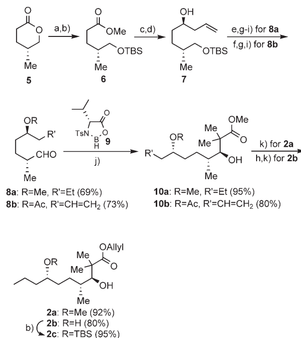
Scheme 2. Synthesis of the HTMMD and the HTMHD unit. a) NaOMe, MeOH, 0°C → RT, 82%; b) TBSCl, imidazole, DMF, 98%; c) DIBAL-H, ether, -90°C; d) [D]B-allyldiisopinocampheylborane, then H 2 O 2 , NaOH, 90% yield for 2 steps; e) NaH, MeI, DMF, RT; f) Ac 2 O, TEA, DMAP, CH 2 Cl 2 , RT; g) TBAF, THF; h) Pt/C, H 2 , EtOAc; i) Swern oxidation; j) 1-(trimethylsiloxy)-1-methoxy-2-methyl-1-propene, borane 9 , CH 2 Cl 2 , -78°C; k) aq. LiOH, THF, MeOH, then allyl bromide, K 2 CO 3 , DMSO, RT. TBS = tert -butyldimethylsilyl; DIBAL = diisobutylaluminum hydride; TBAF = tetrabutylammonium fluoride; DMAP = 4-dimethylaminopyridine.
