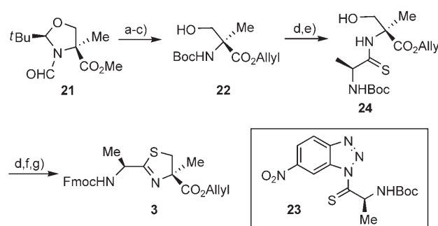
Scheme 7. Synthesis of α-methylthiazoline unit. a) AcCl, MeOH, reflux; b) Boc 2 O, Na 2 CO 3 , THF, H 2 O, RT, 80% yield for 2 steps; c) aq. LiOH, THF, MeOH, then allyl bromide, K 2 CO 3 , DMSO, RT, 94%; d) TFA, CH 2 Cl 2 ; e) 23 , Et 3 N, CH 2 Cl 2 , 0 °C → RT, 50% yield for 2 steps; f) FmocOSu, Na 2 CO 3 , dioxane, H 2 O, 80%; g) DAST, CH 2 Cl 2 , –78 °C, 89%. Fmoc = 9-fluorenylmethoxycarbonyl; DAST = (diethylamino)sulphur tri-fluoride.
