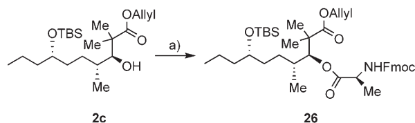
Scheme 9. Synthesis of the ester 26 . a) N -Fmoc-Ala-Cl (5.0 equiv), DMAP (0.5 equiv), i Pr 2 NEt (5.5 equiv), CH 2 Cl 2 , –15 °C, 37% yield, 62% starting material was recovered.
