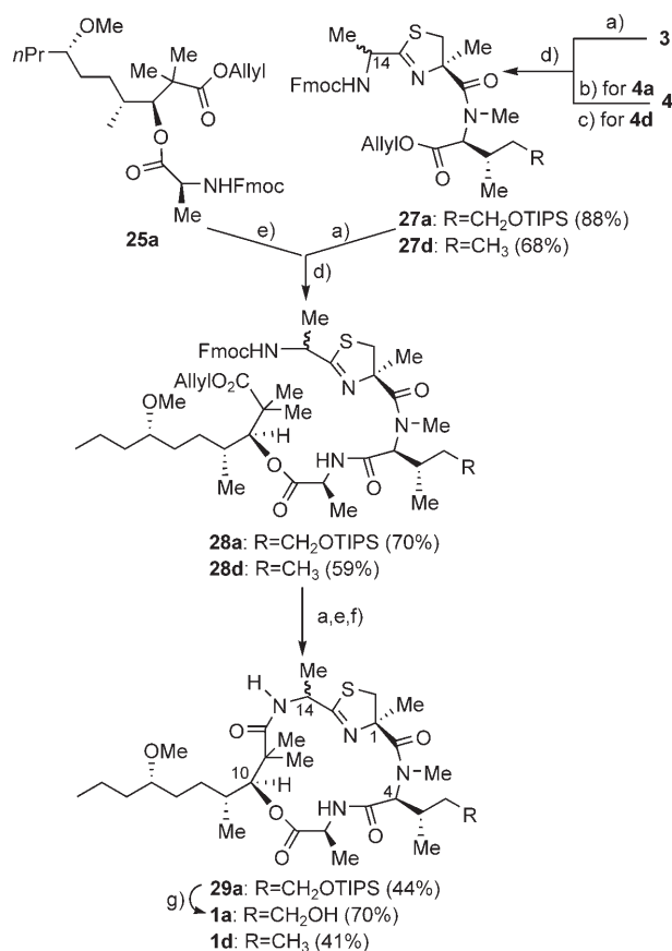
Scheme 10. Completion of syntheses of halipeptins A and D. a) [Pd(PPh 3 ) 4 ], NMA, CH 2 Cl 2 , RT; b) AlCl 3 , CH 2 Cl 2 , 0 °C → RT; c) TFA, CH 2 Cl 2 ; d) BEP, i Pr 2 NEt, CH 2 Cl 2 , 0 °C → RT; e) CH 3 CN, Et 2 NH; f) HATU, i Pr 2 NEt, DMF, CH 2 Cl 2 , 0 °C → RT; g) TBAF, THF, 70%. BEP = 2-bromo-1-ethyl-pyridinium tetrafluoroborate; HATU = N -[(dime-thylamino)-1 H -1,2,3-triazolo[4,5- b ]pyridin-1-yl-methylene]- N -methylme-thanaminium hexafluorophosphate N -oxide.
