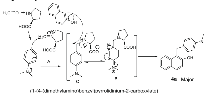
Figure 1. Possible mechanism of reaction.
