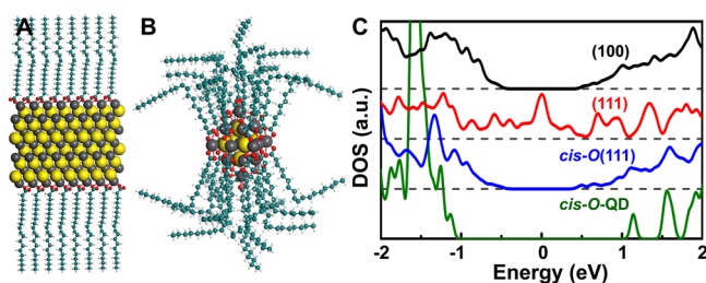
Figure 3. Ball-and-stick models of Pb-rich cis -O(111)-terminated (A) surface and (B) ultrasmall QDs (gray, Pb; yellow, S; red, O; cyan, C; white, H). (C) Calculated electronic DOSs of (100), (111), cis -O(111), and cis -O QDs near the Fermi energy ( E = 0 ).
