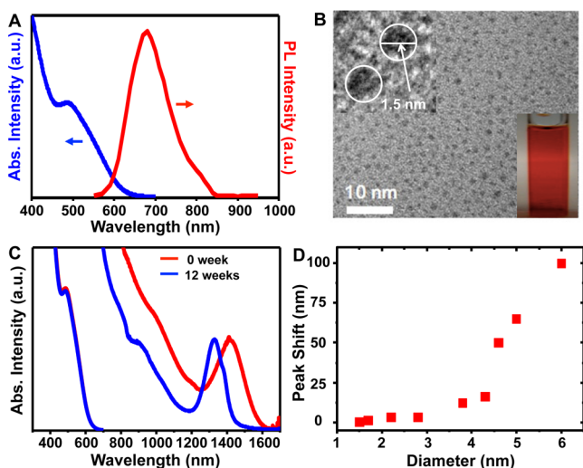
Figure 1. (A) Absorption and photoluminescence spectra of ultrasmall PbS QDs dispersed in tetrachloroethylene. (B) TEM image of the ultrasmall PbS QDs with 1S_{\max} = 480 nm. (Inset) High-resolution TEM image of individual ultrasmall QDs showing D \approx 1.5 nm, and a photograph of a colloidal solution of ultrasmall QDs showing its daylight color is red. (C) Absorption spectra of ultrasmall and large QDs just after synthesis and after 12 weeks of being stored in ambient atmosphere, showing a blue peak shift. (D) Peak shift depending on QD size, showing a transition at \sim 4 nm.
