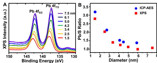
Figure 2. (A) High-resolution Pb 4f XPS spectra of PbS QDs with D = 1.5 –7.5 nm. (B) Diameter-dependent Pb/S atomic ratio of PbS QDs obtained from ICP-AES and XPS.
