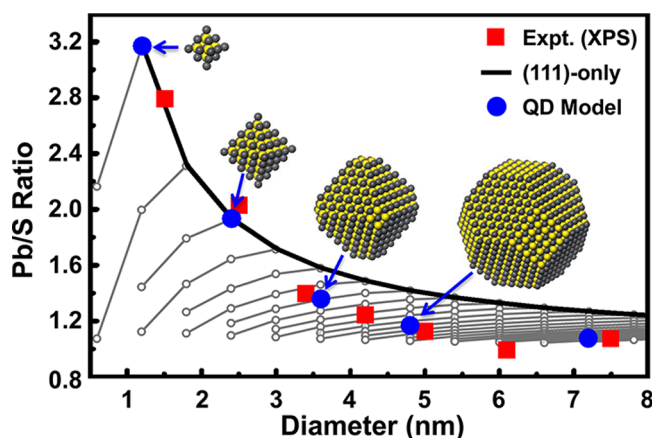
Figure 4. Pb/S ratio of octahedral and cuboctahedral PbS QD models as a function of diameter, compared with the XPS data. The (111)-only octahedral QDs show a deviation from experimental data at D \approx 3 nm. Proposed QD models are shown in the inset data, marked with blue circle.
