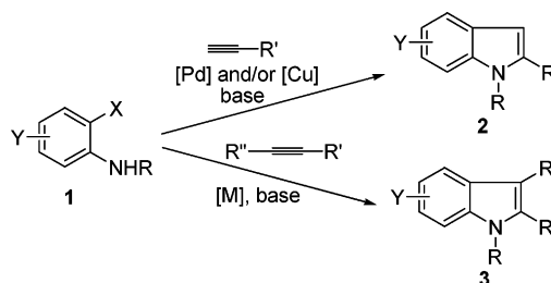
SCHEME 1. Assembly of Indoles via Coupling of o -Haloaniline Derivatives and Alkynes
