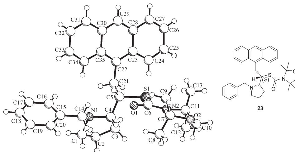
Figure 3. X-ray crystal structure of (S)-23.
