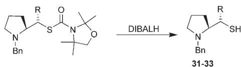
Scheme 5. Decarbamylation of substituted thiocarbamates.
