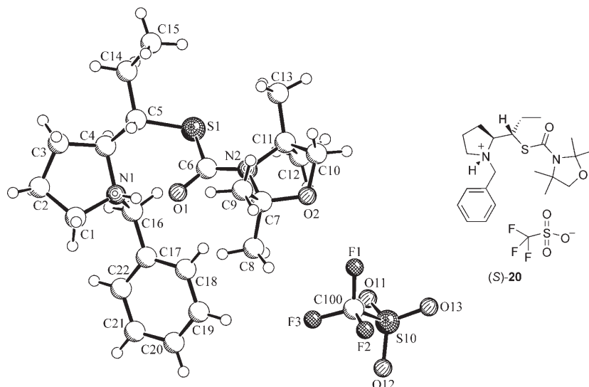
Figure 2. X-ray crystal structure of triflate salt (S)-20. [12]
