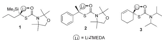
Scheme 1. Configurational stable \alpha -thio-organolithium compounds.
