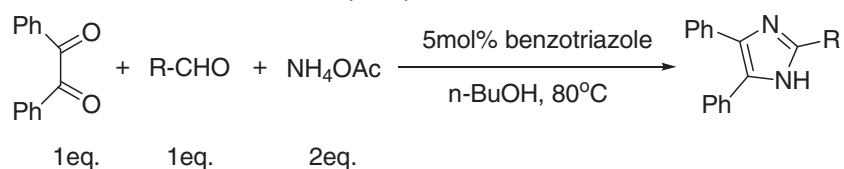
Scheme 2. Benzotriazole-catalyzed synthesis of 2,4,5-trisubstituted imidazoles.
