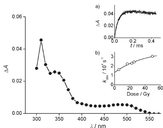
Figure 2. Transient absorption spectrum obtained from the pulse radiolysis of an Ar-purged solution containing 12 (1 mM) and t BuOH (0.25 M) at pH \approx 7, taken 170 \mu s after the pulse; dose = 23.8 Gy, optical path = 2.0 cm. Insets: a) Time-dependence of absorption at \lambda = 310 nm; dose = 22.6 Gy; b) Dependence of k_{\text{obs}} (see text) from the radiation dose at \lambda = 310 nm.
