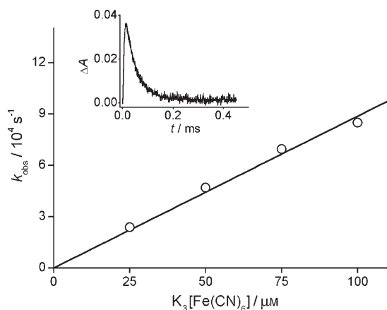
Figure 5. Dependence of k_{\text{obs}} for decay at \lambda=350 \text{ nm} on [\text{K}_3[\text{Fe}(\text{CN})_6]] obtained from the pulse radiolysis of Ar-purged solutions containing 8 (1 mM) and t BuOH (0.25 M) at \text{pH} \approx 7 . Inset: Time-dependence of the absorption at 350 nm in the presence of \text{K}_3[\text{Fe}(\text{CN})_6] (25 \mu\text{M} ); optical path = 2.0 cm, dose = 23.9 Gy. The solid line represents the first-order kinetic fit to the data.
