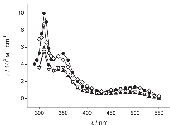
Figure 3. Transient absorption spectra obtained from the pulse radiolysis of solutions containing (●) 8 (1 mM) and t BuOH (0.25 M) at pH ≈ 7, Ar-purged, taken 20 μs after the pulse, assuming G=0.27 \mu\text{mol J}^{-1} and extrapolating to zero dose; (▲) 12 (1 mM) and t BuOH (0.25 M) at pH ≈ 7, Ar-purged, taken 170 μs after the pulse, assuming G=0.27 \mu\text{mol J}^{-1} and extrapolating to zero dose; (▽) taken from ref. [14] and refers to inosine (0.2 mM) and t BuOH (0.1 M) at pH ≈ 7, N 2 O-saturated, taken 40 μs after the pulse; (◇) inosine (2 mM) and t BuOH (0.2 M) at pH ≈ 7, N 2 O-saturated, taken 9 μs after the pulse, dose = 19.6 Gy, assuming G=0.084 \mu\text{mol J}^{-1} .
