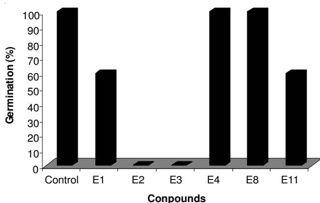
Fig. 1. Phytotoxicity of synthetic compounds on canola ( Brassica napus L.) seed germination. Compounds: Methyl-2,3-diacetoxy-4-oxo-4-(4'-bromophenyl amino)butanoate (MES- E3 ), methyl-2,3-diacetoxy-4-oxo-4-(4'-trifluoromethyl phenyl amino) butanoate (MES- E8 ), methyl-2,3-diacetoxy-4-oxo-4-(2'-trifluoromethyl phenyl amino)butanoate (MES- E4 ), methyl-2,3-diacetoxy-4-oxo-4-(2'-bromophenyl amino)butanoate (MES- E2 ), methyl-2,3-diacetoxy-4-oxo-4-(4'-methyl phenyl amino)butanoate (MES- E1 ), methyl-2,3-diacetoxy-4-oxo-4-(2'-methoxyphenylamino)butanoate (MES- E11 )
