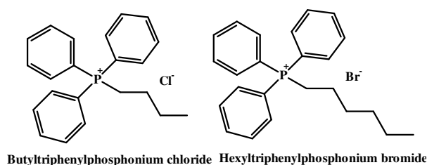
Fig. 1. Structures of ionic liquids used in this study
