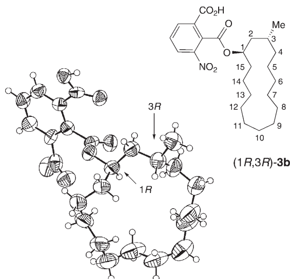
Figure. X-Ray crystal-structure (ORTEF plot) of 2-[(1 R ,3 R )-3-methylcyclopentadecyl] hydrogen 3-nitrobenzene-1,2-dicarboxylate ((1 R ,3 R )- 3b ). Ellipsoids are represented at the 50% probability level.
