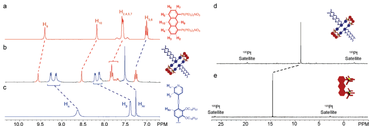
FIGURE 1. Representative 1 H NMR spectra (300 MHz, 298 K, CD 3 COCD 3 ) of the aromatic portion of the (a) molecular clip, (b) hydrophobic molecular C 18 Rectangle 16, (c) and hydrophobic C 18 donor 10 displaying the characteristic shifts of proton signals associated with the donor and acceptor units upon coordination as well as (d) the 31 P { 1 H} NMR spectra of the self-assembled C 18 Rectangle 16 and (e) molecular clip.
