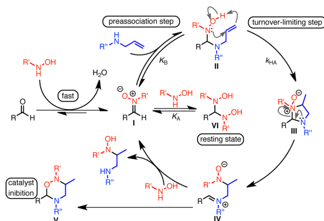
Figure 7. Proposed catalytic cycle.
