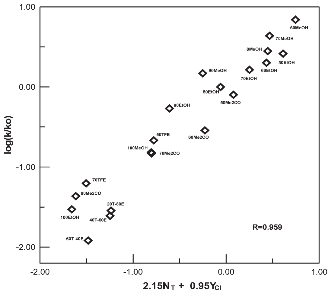
Figure 1. Plot of \log(k/k_o) for solvolyses of 2-adamantyl fluoroformate in pure and binary solvents at 25.0°C against (2.15N_T + 0.95Y_{Cl})
