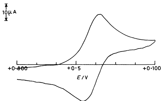
Figure 6. Cyclic voltammogram recorded at a platinum electrode on a deaerated acetonitrile solution containing [\text{CuL}_6]^{2+} ( 1.00 \times 10^{-3} \text{ mol dm}^{-3} ). Scan rate 0.5 \text{ V s}^{-1}
