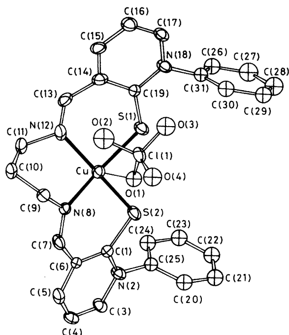
Figure 1. ORTEP diagram of [CuL^2(ClO_4)]^+ with atomic labelling. Thermal ellipsoids are drawn at 30% probability. Hydrogen atoms are omitted for clarity.
