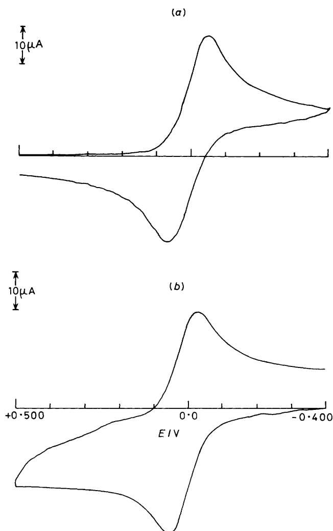
Figure 2. Cyclic voltammograms recorded at a platinum electrode on deaerated acetonitrile solutions containing \text{NEt}_4\text{ClO}_4 ( 0.1 \text{ mol dm}^{-3} ) and (a) [\text{CuL}^2]^{2+} ( 1.40 \times 10^{-3} \text{ mol dm}^{-3} ), (b) [\text{CuL}^2]^+ ( 1.30 \times 10^{-3} \text{ mol dm}^{-3} ). Scan rate 0.5 \text{ V s}^{-1} .
