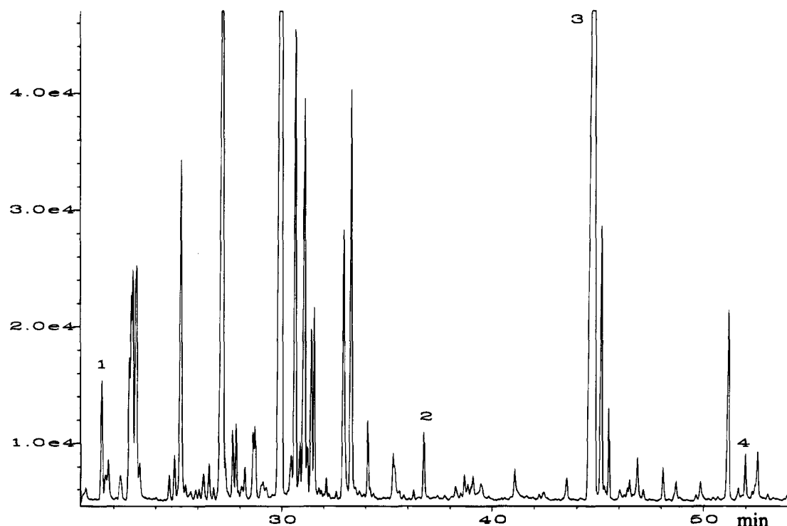
Figure 2. Gas chromatogram of fraction E separated on a 60 m \times 0.32 mm (i.d.) DB-1 column. Fraction E was obtained by separation of used oil volatiles by silica gel column chromatography. Peaks 1, 2, 3, and 4 represent 4-oxohexanal, 4-oxooctanal, 4-oxononanal, and 4-oxodecanal, respectively.
