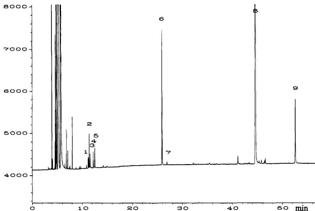
Figure 1. Gas chromatogram of products formed from the thermal treatment of 4-oxononanal. Temperature was programmed from 30 (4 min isothermal) to 200 °C at 2 °C/min on a 60 m \times 0.32 mm (i.d.) DB-1 column. The peak numbers correspond to the numbers in Table 1.
