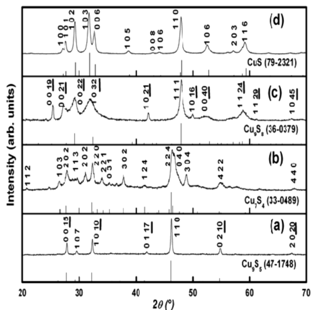
Figure 2. Powder X-ray diffraction pattern of (a) \text{Cu}_9\text{S}_5 , (b) \text{Cu}_7\text{S}_4 , (c) \text{Cu}_9\text{S}_8 , and (d) \text{CuS} obtained from the reaction of \text{Cu}_2\text{S} with 0.20, 0.25, 0.88, and 1 mol of iodine solution in acetonitrile for 2 days at 25 °C.
