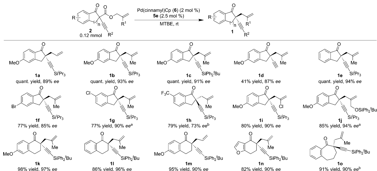
Scheme 2. Scope of the Pd-Catalyzed Decarboxylative Allylation a
