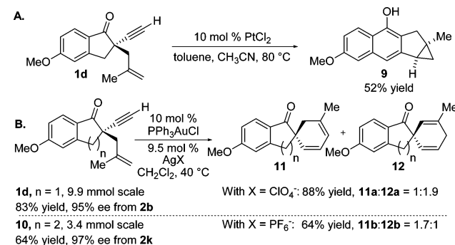
Scheme 4. Au- and Pt-Catalyzed Cycloisomerizations
