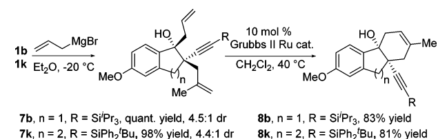
Scheme 3. Synthesis of Fused Ring Systems
