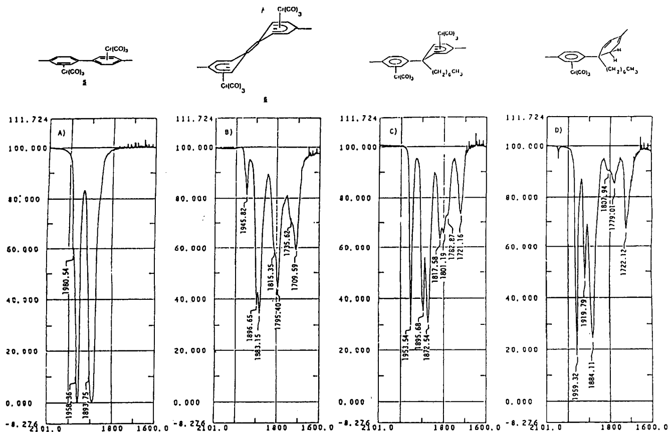
Figure 1. Infrared carbonyl stretching bands ( \text{cm}^{-1} ) for (\eta^6:\eta^6\text{-4,4'-dimethylbiphenyl})\text{bis}(\text{tricarbonylchromium}) in THF: (A) before reduction; (B) after reduction with lithium naphthalenide; (C) after alkylation of the reduced species with 1 equiv of heptyl iodide; (D) after protonation of the alkylated species with 1 equiv of trifluoroacetic acid.
