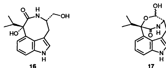
Scheme 4 Reagents and conditions: i, \text{SO}_2\text{Cl}_2 , heat; ii, tert -BuOCl, \text{CH}_2\text{Cl}_2 ; iii, (L)-Trp-OMe, aq. \text{NaHCO}_3 , \text{CH}_2\text{Cl}_2 ; iv, h\nu , MeCN; v, h\nu , aq. MeCN
