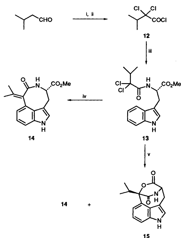
Scheme 4 Reagents and conditions: i, \text{SO}_2\text{Cl}_2 , heat; ii, tert -BuOCl, \text{CH}_2\text{Cl}_2 ; iii, (L)-Trp-OMe, aq. \text{NaHCO}_3 , \text{CH}_2\text{Cl}_2 ; iv, h\nu , MeCN; v, h\nu , aq. MeCN
