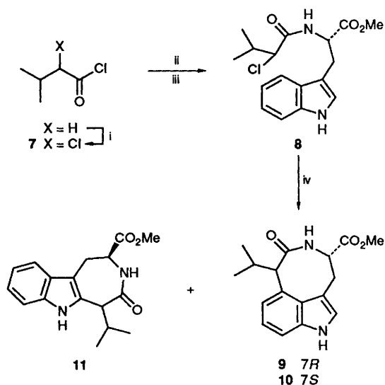
Scheme 3 Reagents and conditions: i, N -chlorosuccinimide, \text{SOCl}_2 , heat; ii, (L)-Trp, NaOH; iii, \text{CH}_2\text{N}_2 ; iv, h\nu , MeCN
