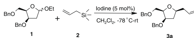
Scheme 1. Preparation of product 3a .
