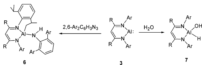
Scheme 3. Reaction of 3 with 2,6-Ar 2 C 6 H 3 N 3 and H 2 O
