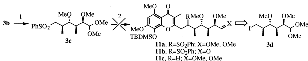
Scheme 5. Reagents and conditions: (1) oxone (5 equiv.), pH 8–9 phosphate buffer, MeOH; 0^{\circ}\text{C} , 4 h (80%); (2) n -BuLi (1.3 equiv.), HMPT (1.3 equiv.), THF; -78^{\circ}\text{C} to rt
