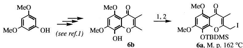
Scheme 2. Reagents and conditions: (1) TBDMSCl (2.5 equiv.), imidazole (2.5 equiv.); DMF, rt, 15 h (73%); (2) LDA (1 equiv.), THF; -78°C, 1 h, then NIS (1.5 equiv.), -78°C, 2 h (37% overall, from 6b )
