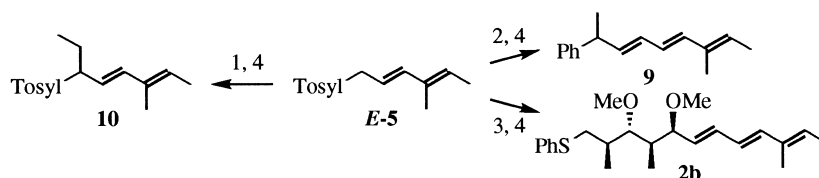
Scheme 4. Reagents and conditions: (1) 1.2 M (in hexane) n -BuLi (1.05 equiv.), THF; -78 to 35^{\circ}\text{C} , 15 min, then -78^{\circ}\text{C} , 0.5 h, then acetaldehyde (1.3 equiv.); -78 to -20^{\circ}\text{C} , 15 min; (2) same conditions as in (1) with 2-phenylpropanal; (3) same conditions as in (1) with the aldehyde 3a ; (4) (i) Ac 2 O (2.1 equiv.), DMAP (0.11 equiv.), rt, 1 h; (ii) 6% HgNa (400 mg/mmol, three times), HNa 2 PO 4 ·12H 2 O (3×4 equiv.), MeOH; -20^{\circ}\text{C} , 5–7 h
