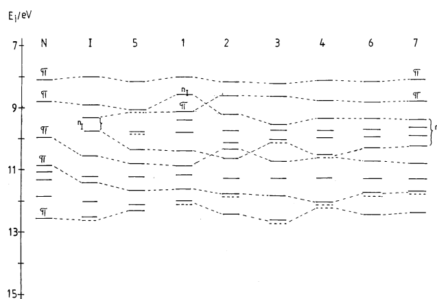
Figure 5. Energy level diagram for diiodonaphthalenes.
