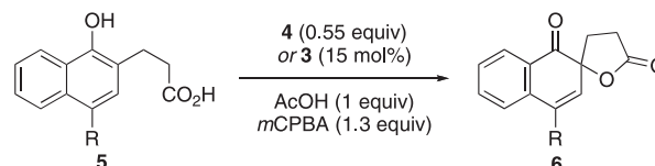
Scheme 1. Enantioselective oxidative spirolactonization of 1-naphthols ( 5 ) reported by Kita and co-workers. 6
