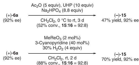
Scheme 8. Epoxidation of (+)-6a to epoxyspirolactone (-)-15 .
