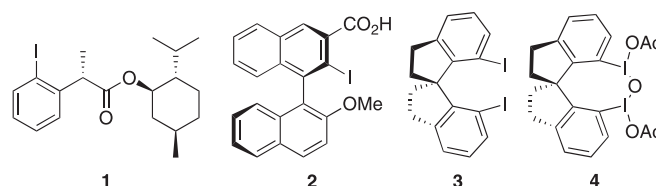
Figure 1. Chiral iodoarene precatalysts 1–3 and iodosylarene 4 .
