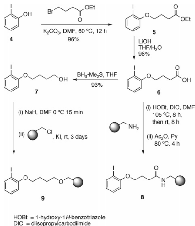
SCHEME 2. Oxidation of Resins 8 and 9
