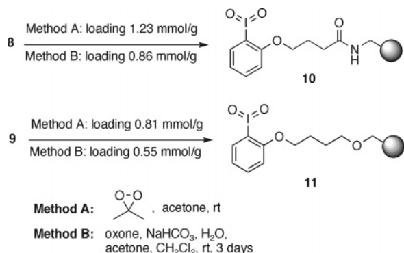
SCHEME 2. Oxidation of Resins 8 and 9
