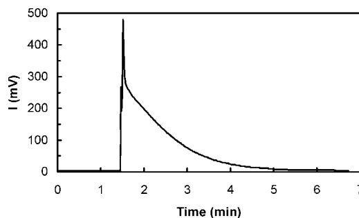
FIGURE 3. IR luminescence signal of ^1\text{O}_2 generated by a solution containing 0.01 M PIFA, 0.1 M \text{NaHCO}_3 , and 0.1 M rac -1-phenylethyl hydroperoxide (7) in toluene at T = 20 °C.
