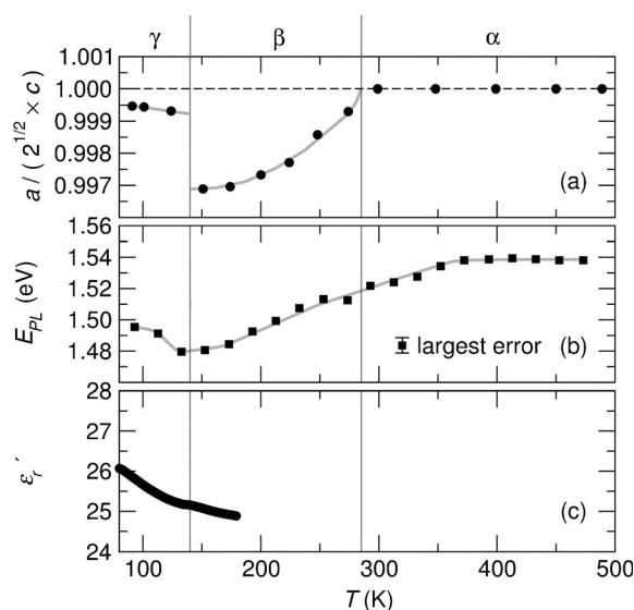
Figure 3. Tetragonal lattice parameter ratio, photoluminescence peak energy, and static dielectric permittivity of \text{HC}(\text{NH}_2)_2\text{PbI}_3 . a) The tetragonal lattice parameter ratio reflects the continuous \alpha - \beta transition on cooling, as well as the reentrant cubic pseudosymmetry in the \gamma -phase. Error bars are smaller than the markers and are omitted. b) The photoluminescence (PL) emission peak energy, E_{\text{PL}} , red-shifts on warming through the \gamma - \beta transition. In the \beta - and \alpha -phases, E_{\text{PL}} blue-shifts with temperature, consistent with the effects of lattice expansion [11] on the unusual electronic structure of the main-group halide perovskites, and subsequently plateaus above 370 K. c) Static dielectric permittivity, \epsilon' , extracted from capacitance-loss measurements at 20 kHz. Despite a slight kink at the \beta - \gamma transition, \epsilon' declines substantially with temperature in both phases, suggesting reorientation of the dipolar axis of the A-site cation is minimally inhibited even at these temperatures.
