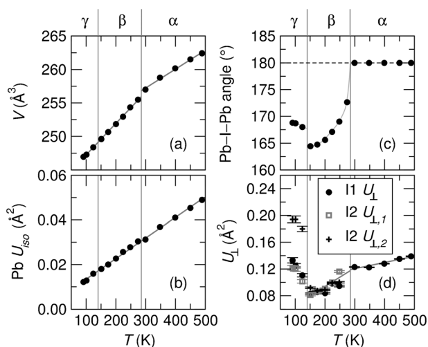
Figure 4. Selected crystallographic parameters for \text{HC}(\text{NH}_2)_2\text{PbI}_3 . Error bars for (a)–(c) are smaller than the markers and are omitted. a) The unit cell volume per formula unit, V , reveals unusually large volumetric thermal expansion coefficients ( \alpha_v = 203 \times 10^{-6} \text{ K}^{-1} at 274 K). \alpha_v is reduced in the cubic phase, consistent with a negative contribution from large amplitude dynamic octahedral tilts. [16–18] b) The isotropic ADP for Pb, U_{\text{iso}} , is large compared to typical values in oxides but reveals no discontinuities associated with masked displacements in the tetragonal phases. c) The Pb-I-Pb octahedral tilt angle reflects the continuous \alpha - \beta transition, and jumps back toward linear through the unusual \beta - \gamma transition. d) The ADPs for I in the directions orthogonal to the Pb-I bonds, U_{\perp} , decline monotonically with cooling in the \alpha - and \beta -phases, consistent with reduced dynamic octahedral tilting. The increased values of the U_{\perp} ADPs on cooling to the \gamma -phase suggest disorder that is not fully captured by this crystallographic model.
