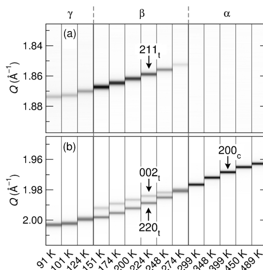
Figure 1. X-ray scattering intensity from \text{HC}(\text{NH}_2)_2\text{PbI}_3 around selected low-angle Bragg peaks between 90 K and 490 K, normalized to maximum peak intensity. a) The 211 t tetragonal Bragg peak emerges upon cooling through a continuous phase transition around 285 K from the cubic \alpha -phase to the tetragonal \beta -phase. b) The 200 c cubic Bragg peak splits continuously on cooling due to the emergent tetragonality. A first-order transition to the pseudo-cubic \gamma -phase with tetragonal symmetry occurs at 140 K. [5] The 002 t and 220 t tetragonal peaks “fuse” across the \beta – \gamma transition while the 211 t tetragonal peak remains.
