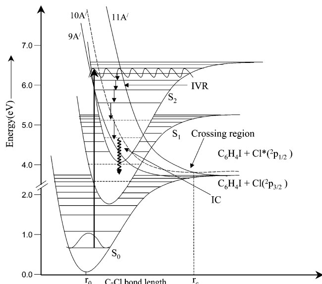
Figure 3. Schematic potential energy diagram describing the mechanism of the C–Cl bond dissociation. IVR is intramolecular vibrational relaxation, and IC, internal conversion. Under C_s geometry, 9A' , 10A' , and 11A' are the (\sigma^*(C-Cl) \leftarrow n(Cl)) transitions.
