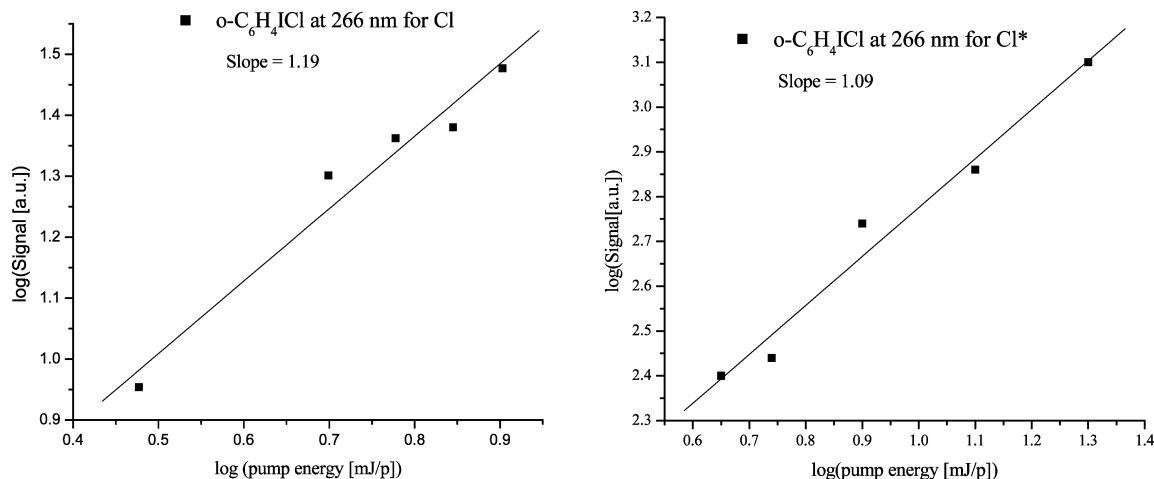
Figure 2. Pump laser power dependence of Cl/Cl* REMPI signal from o-C 6 H 4 I. The straight line is a linear least-squares fit through the experimental points. The slope of the lines is mentioned inside the plots.
