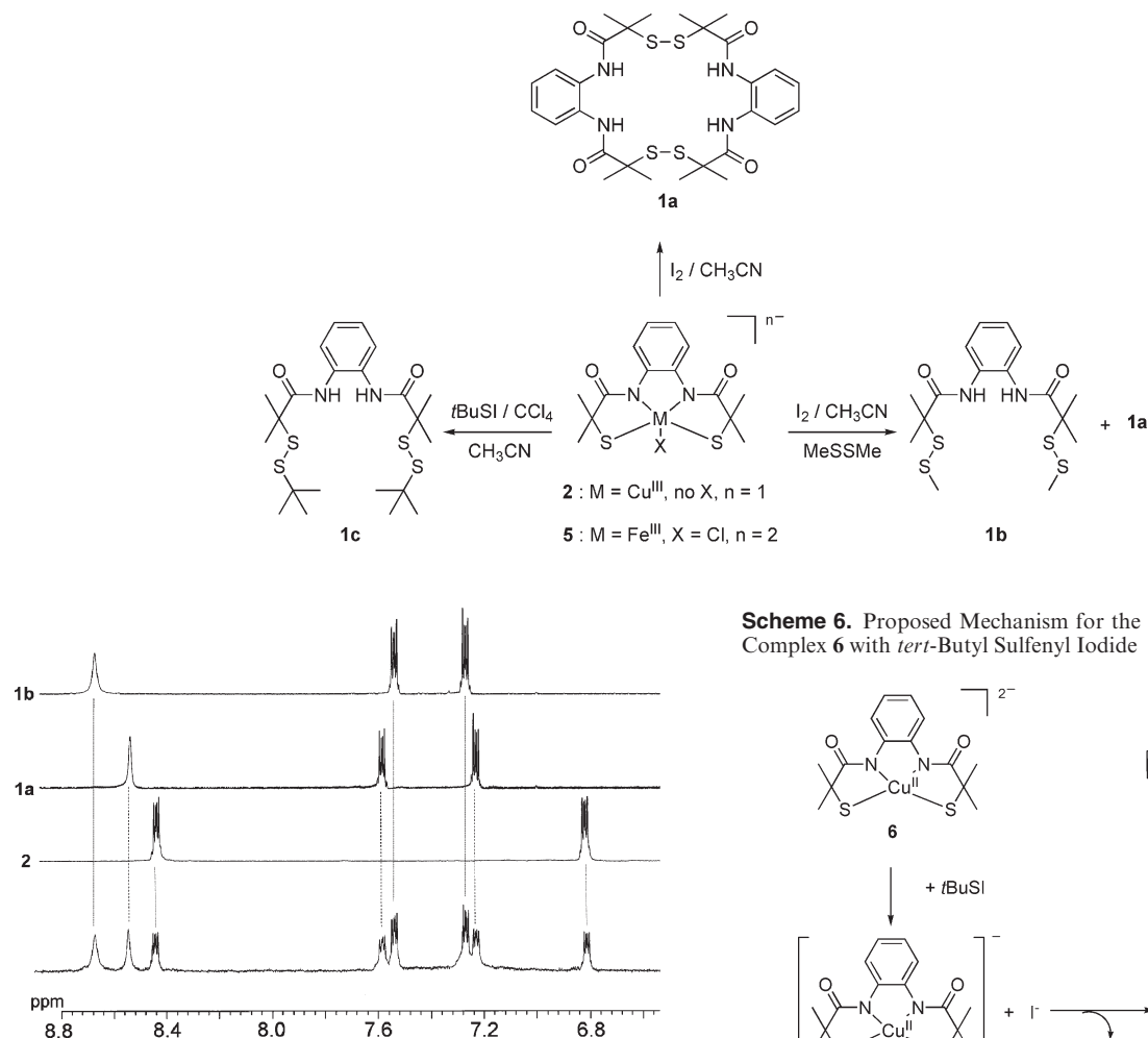
Figure 2. Typical ^1\text{H} NMR spectra, recorded at 500 MHz, obtained after addition of 1 equiv of dimethyl disulfide and 2 equiv of iodine to a 0.04 M solution of complex 2 in \text{CD}_3\text{CN} (bottom), along with the spectra of the authentic compounds 1a , 1b and 2 for comparison (top).
